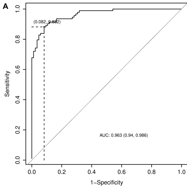
Figure 1. A. ROC curve for PASDAS with MDA state (5/7) as the discriminator. The value of PASDAS when Youden index was maximized (0.80) was 3.2. At this point, the sensitivity was 88% (95% CI 80–93), the specificity was 92% (95% CI 84–96), and the AUC was 0.96 (95% CI 0.94–0.99). B. ROC curve for PASDAS with MDA 6/7 state as the discriminator. The value of PASDAS when Youden index was maximized (0.74) was 2.6. At this point, the sensitivity was 88% (95% CI 82–93), the specificity was 86% (95% CI 74–93), and the AUC was 0.92 (95% CI 0.88–0.96). C. ROC curve for PASDAS with MDA 7/7 state as the discriminator. The value of PASDAS when Youden index was maximized (0.70) was 2.1. At this point, the sensitivity was 89% (95% CI 83–93), the specificity was 81% (95% CI 60–92), and the AUC was 0.91 (95% CI 0.86–0.96). ROC: receiver-operating characteristic; AUC: area under the curve; PASDAS: Psoriatic Arthritis Disease Activity Score; MDA: minimal disease activity.
