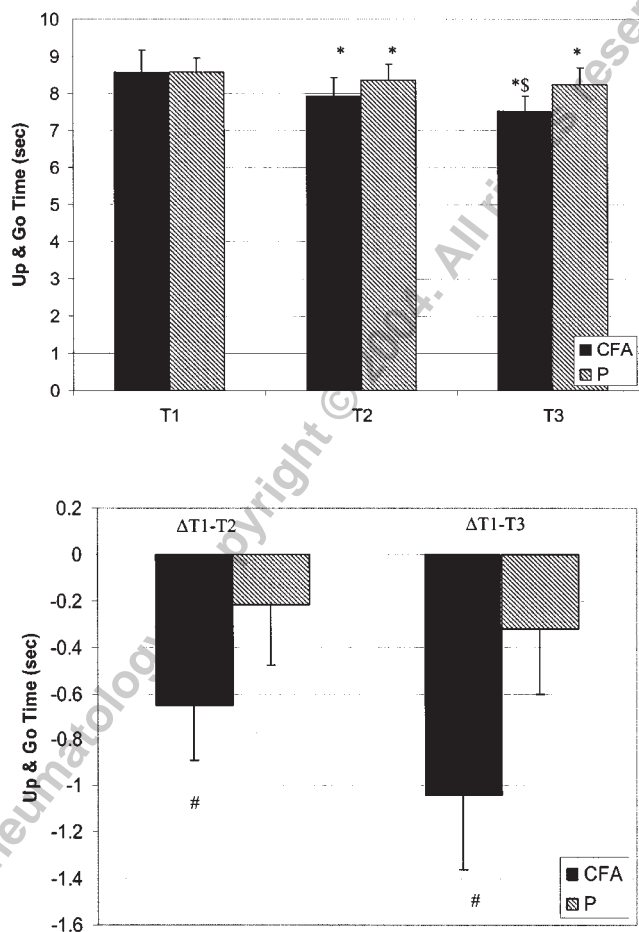
Figure 1. The timed up-and-go assessment in patients using the CFA topical cream or placebo (P). Top panel: the main effects at T1, T2, and T3. Bottom panel: group interactions in differences from T1 to T2 and from T1 to T3. Data are means ± SE. T1: baseline; T2: acute response to initial cream application; T3: post 30-day treatment period. * p < 0.05 from corresponding time point T1. # p < 0.05 between groups. § p < 0.05 from corresponding time point T2.
