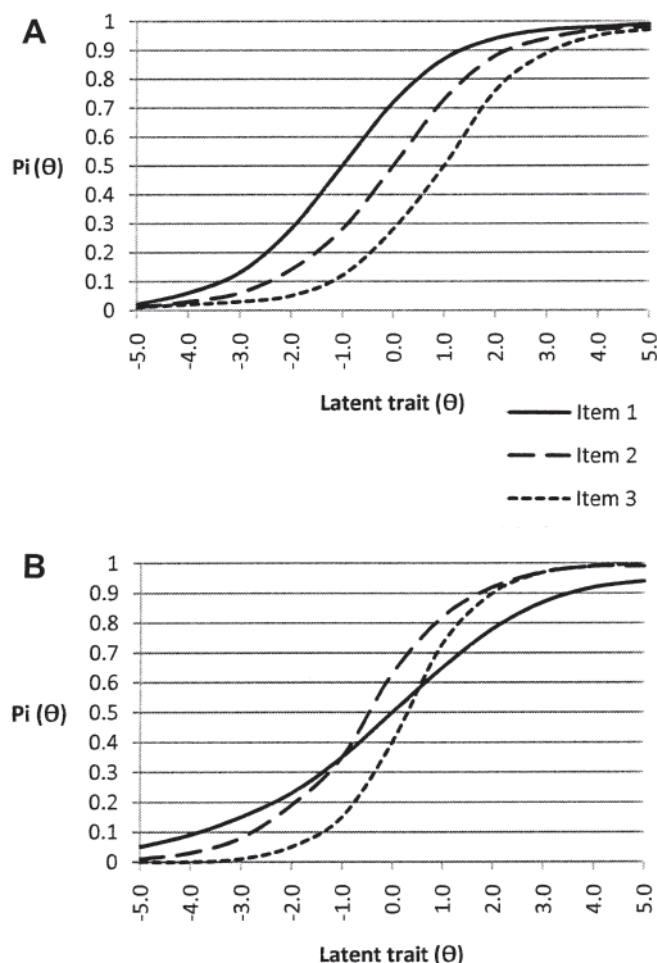
Figure 1. Graphic representation of the Rasch model (A) and the 2-parameter logistic model (B), where P_i(\theta) is the probability of a joint being scored as tender.
