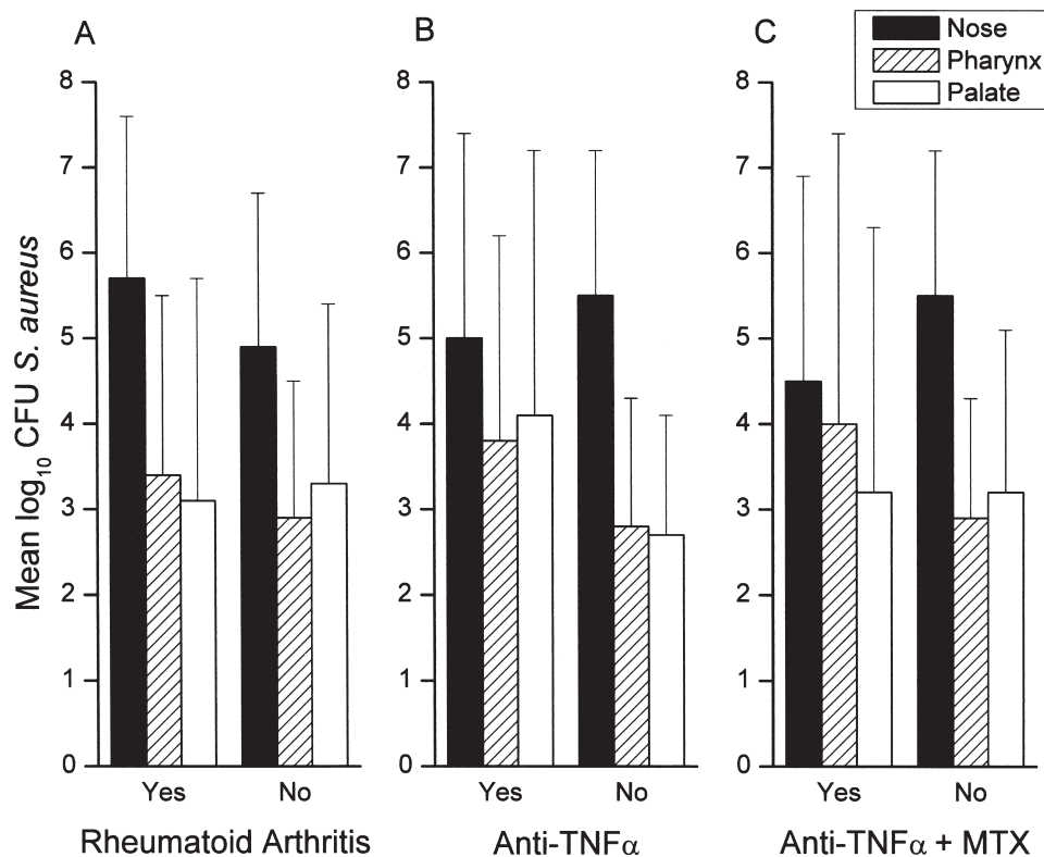
Figure 1. Results of quantitative cultures. Mean log 10 ± SD of CFU of S. aureus in the nose and posterior pharynx and on the soft palate in S. aureus carriers with or without rheumatoid arthritis (A); in S. aureus carriers with or without anti-TNF- \alpha therapy (B); and in S. aureus carriers with or without therapy with an anti-TNF- \alpha agent and methotrexate (C).
