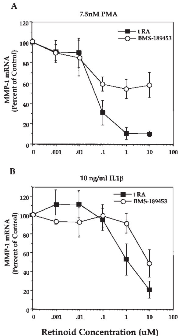
Figure 2. Retinoic acid (tRA) and BMS-189453 inhibition of MMP-1 induction by PMA (A) and IL-1 \beta (B) in HIG-82 rabbit synovial fibroblasts in culture. The standard deviation is indicated by the vertical bar ( n = 4 ).
